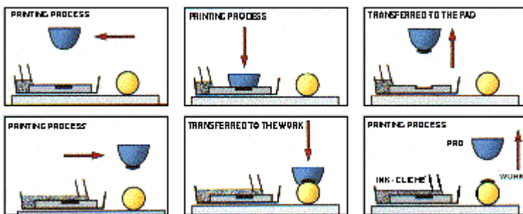
Figure 1: Principles of pad printing
